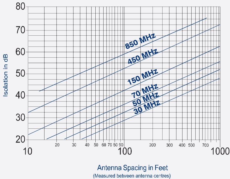
Attenuation provided by HORIZONTAL separation of dipole antennas
