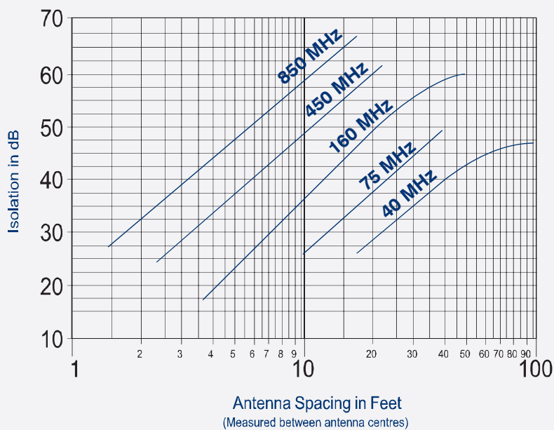
Attenuation provided by VERTICAL separation of dipole antennas
